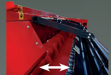
The throughput of the crop can be hydraulically controlled thanks to the height-adjustable reel and the adjustable reel speed.
