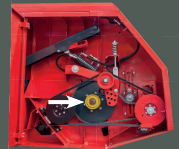
Main driving components are protected with torque limiters.
